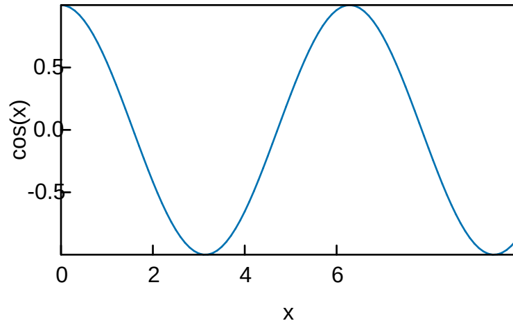
Cosine Wave
