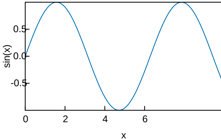
Sine Wave
