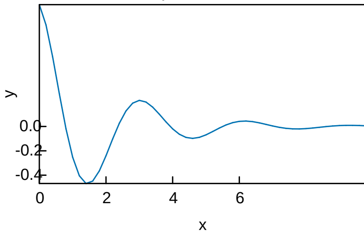
Damped Oscillation
