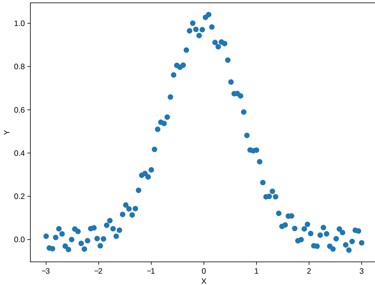
2D Scatter Plot - Gaussian Distribution
