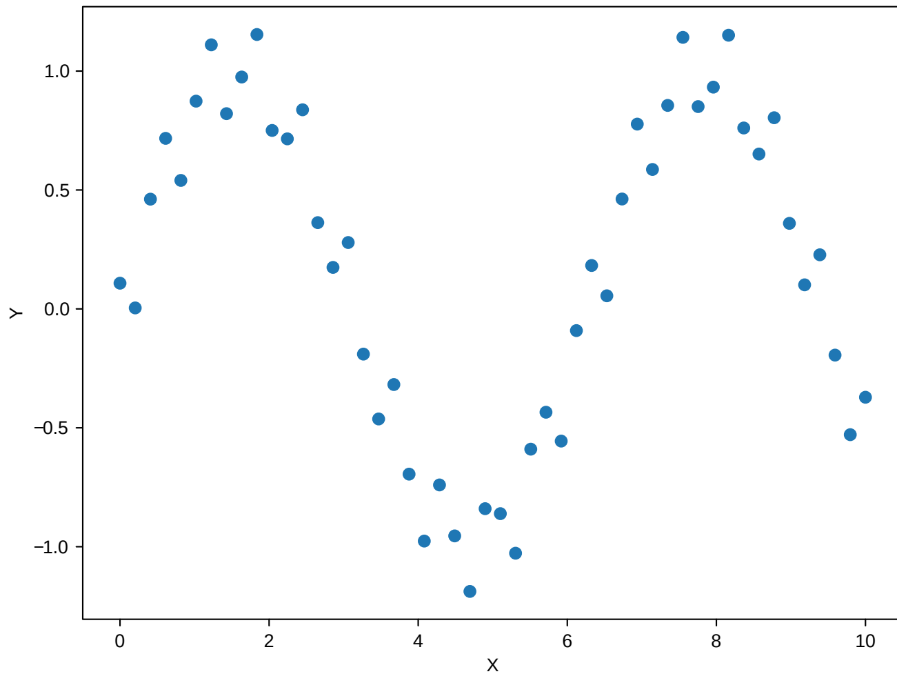
Basic 2D Scatter Plot
