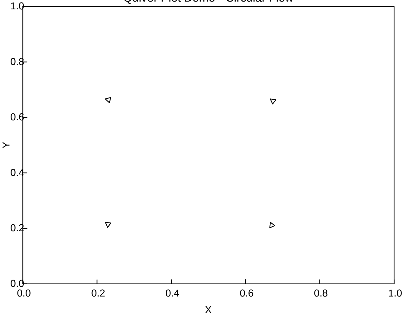
Quiver Plot Demo - Circular Flow
