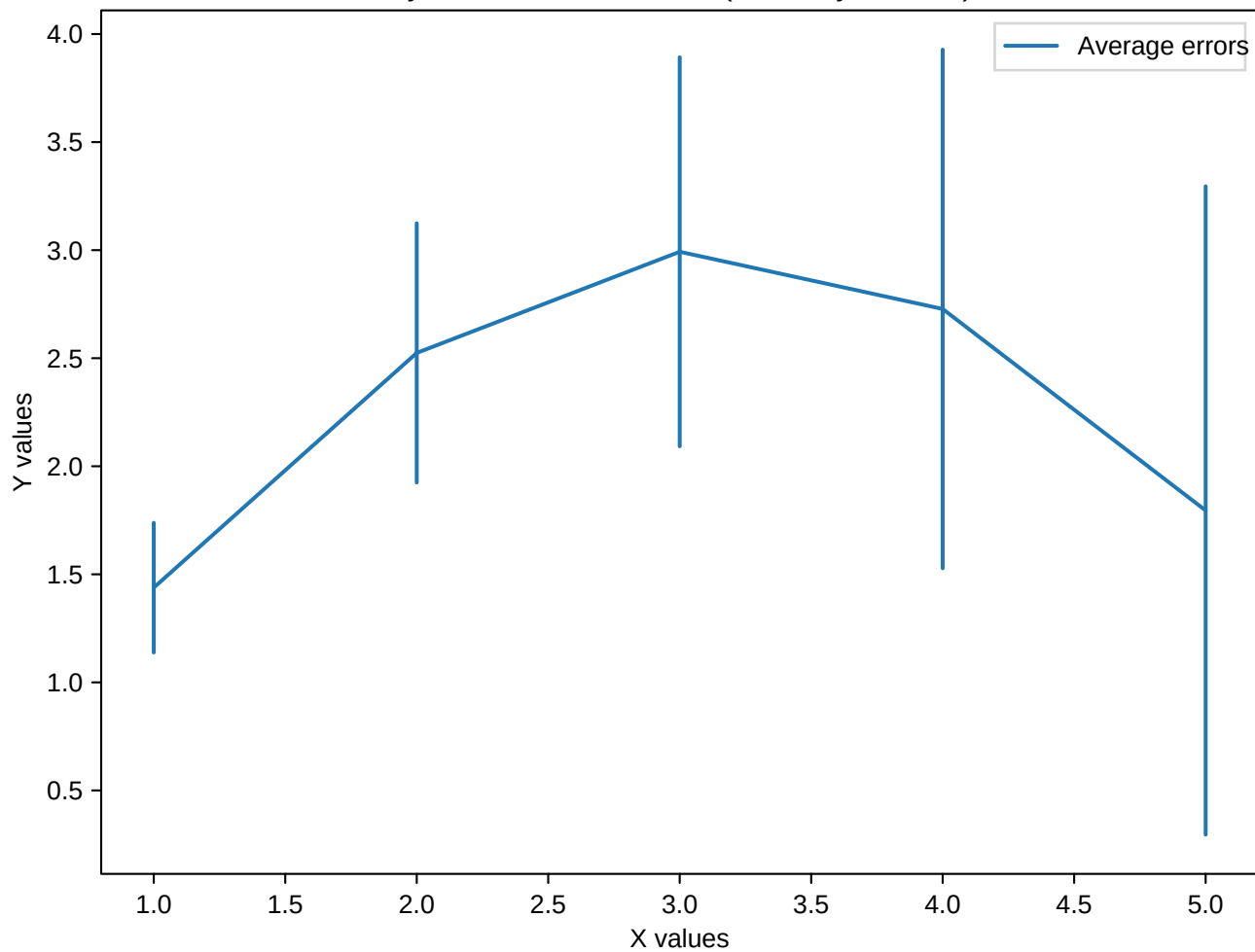
Symmetric Y Error Bars (from asymmetric)
