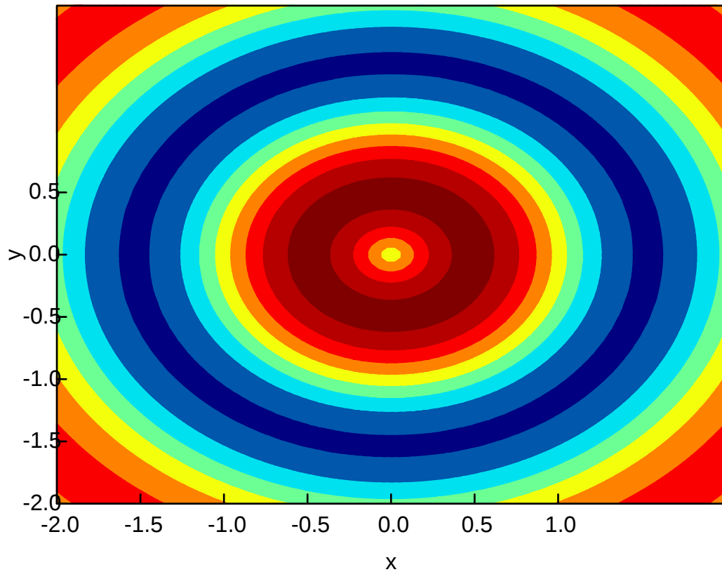
Ripple Function - Jet Colormap
